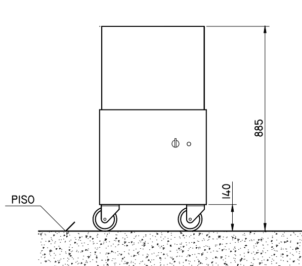
VISTA FRONTAL
