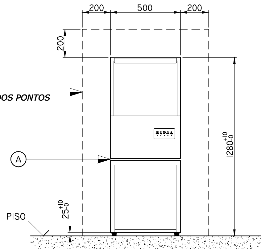
VISTA FRONTAL
