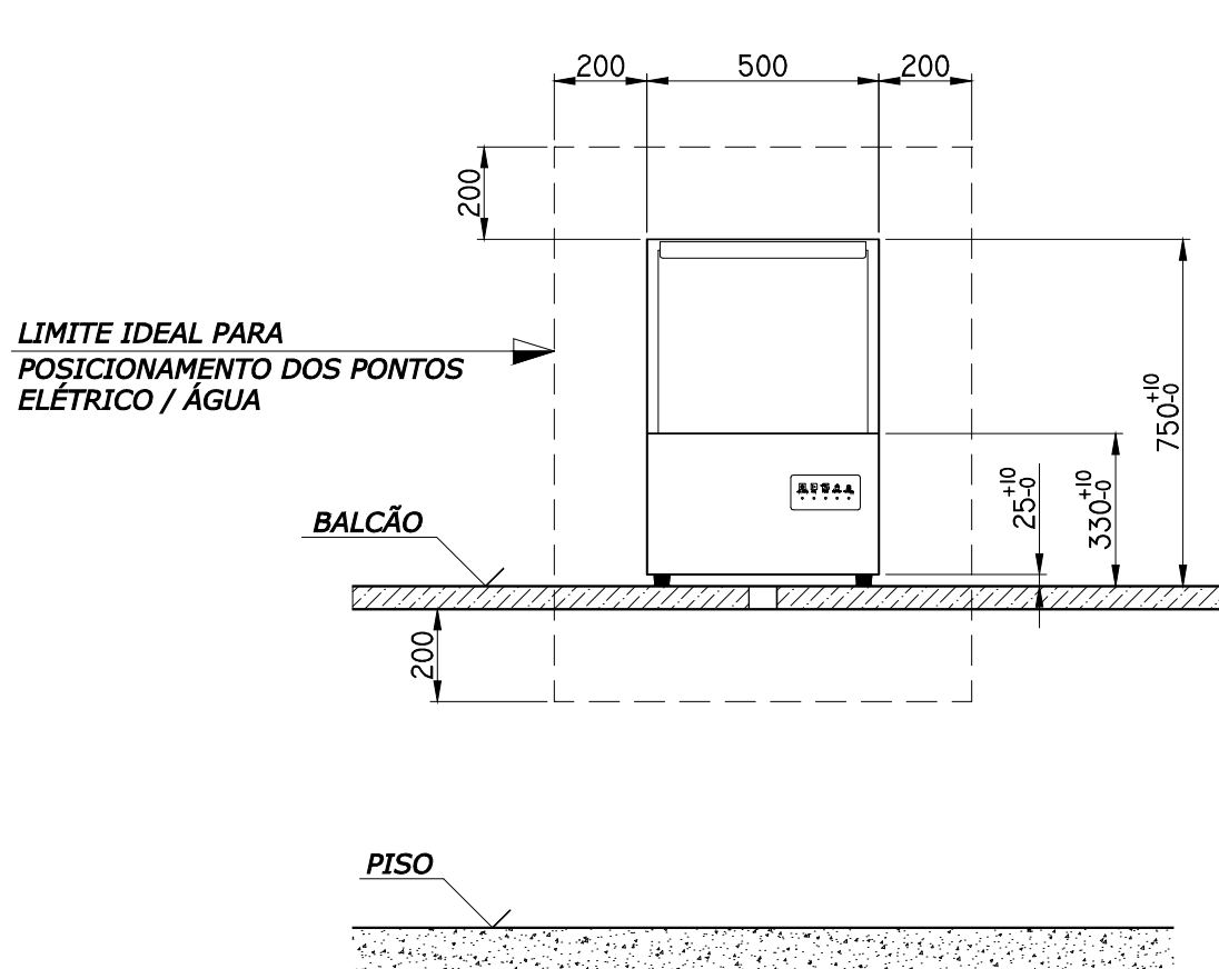
VISTA FRONTAL
